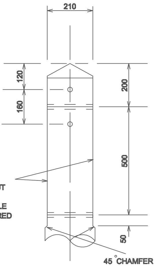
DETAIL A' ' SCALE 1:10
