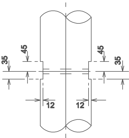
DETAIL B' ' SCALE 1:10
